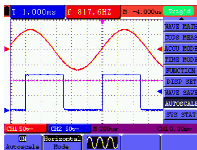
figure 55: only under horizontal mode multi-period waveform
