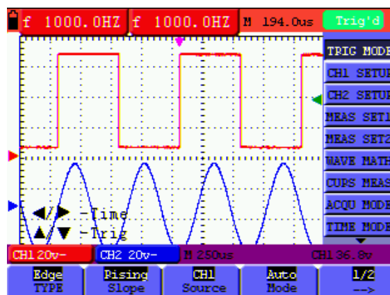
figure 38: Edge Trigger
