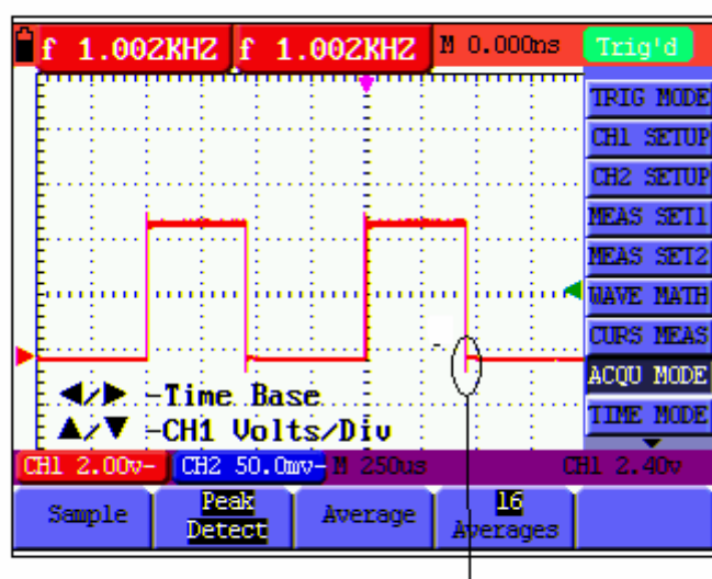
figure 16: Peak Detection
