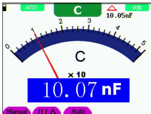
figure 32: Relative Measurement
