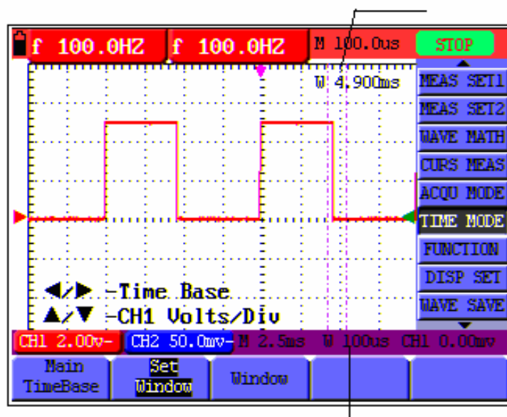
figure 57: Window Setting
