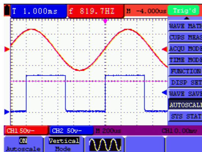
figure 54: only under vertical mode multi-period waveform
