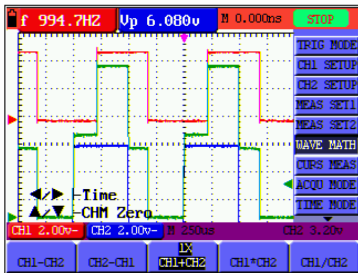
figure 19: Waveform Mathematics
